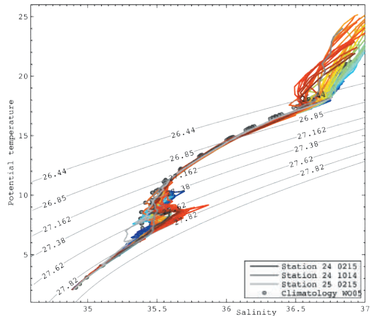
5 POTENTIAL TEMPERATURE/SALINITY DIAGRAM AFTER CALIBRATION.
