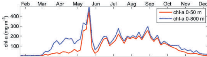
7 VERTICAL SUM OF CHLOROPHYLL-A FLUORESCENCE IN THE UPPER 50 AND 800 M.
