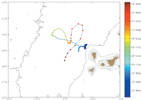
4 TRAJECTORY OF THE E-AIMS DEEP ARVOR FLOAT.
