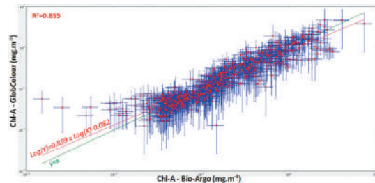
18 COMPARISON OF BIO-ARGO AND SATELLITE CHL-A OBSERVATIONS (875 MATCHUPS).
