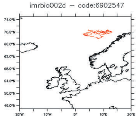
23 COMPARISON OF CHLOROPHYLL-A OBSERVATIONS FROM IMR E-AIMS BIO-ARGO FLOAT WITH THE MERCATOR OCEAN/CMEMS GLOBAL BIOGEOCHEMICAL MODEL.
