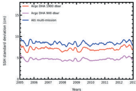
17 STANDARD DEVIATION OF THE ALTIMETER SLA (BLUE) AND THE IN-SITU DYNAMIC HEIGHTS FROM ARGO PROFILES WITH A 900 DBAR REFERENCE (MAGENTA) AND 1,900 DBAR REFERENCE (RED) IN THE ANTARCTIC CIRCUMPOLAR CURRENT.
