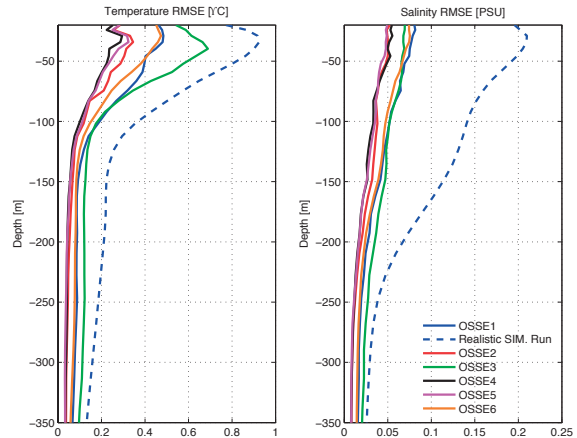
15 RMSE OF THE ARGO MISFIT DURING THE 2012 FOR ALL THE MEDITERRANEAN SEA. BLUE LINE OSSE1 (5 DAYS DRIFT, PD 350M), RED LINE OSSE2 (5 DAYS DRIFT, PD 700M), GREEN LINE OSSE3 (5 DAYS DRIFT, PD 150M), BLACK LINE OSSE4 (3 DAYS DRIFT, PD 350 M) MAGENTA LINE OSSE5 (3 DAYS DRIFT, PD 700M) AND ORANGE LINE OSSE6 (5 DAYS DRIFT, PD 350 M, PERFECT VERTICAL SAMPLING).
