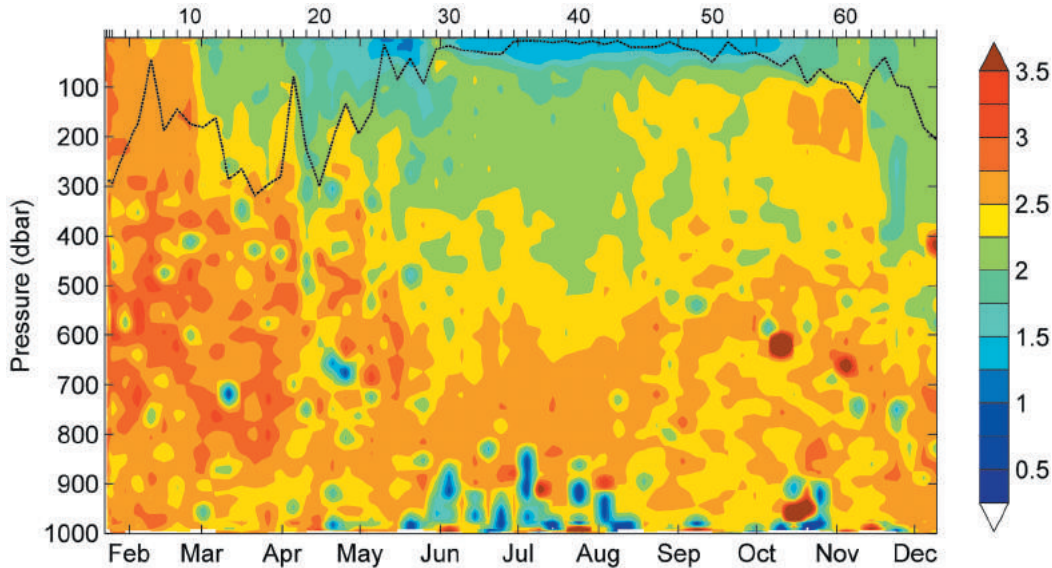
8 RATIO OF PARTICULATE BACKSCATTERING (BBP532:BBP700) AS A FUNCTION OF DEPTH AND TIME. THE SOLID BLACK LINE IS THE MIXED-LAYER DEPTH.
