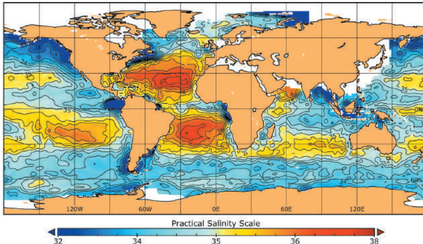
19 SEA SURFACE SALINITY - 1X1 OPTIMAL INTERPOLATION MAP - 17/26 FEBRUARY, 2012 - BEC PRODUCT
