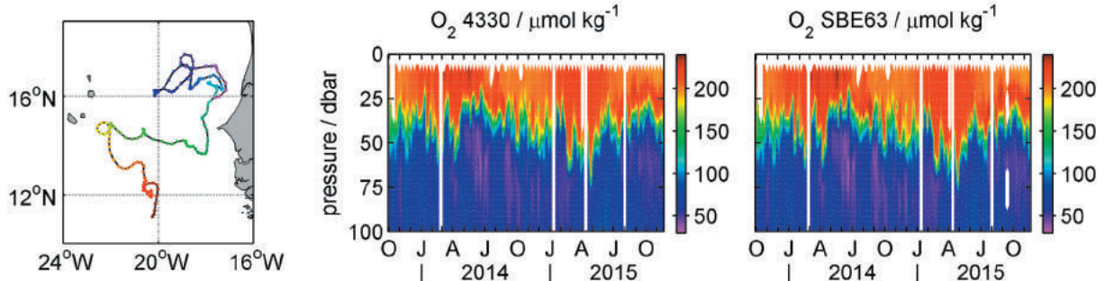
2 OXYGEN PROFILES MEASURED WITH THE AANDERAA AND THE SBE63 OPTODES FOR THE NAVIS FLOAT F0271.
