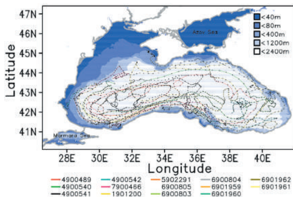
16 TRAJECTORIES OF THE ARGO FLOATS USED IN THE ANALYSIS IN THE BLACK SEA.
