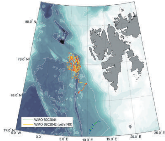
10 TRAJECTORIES OF THE TWO E-AIMS ARCTIC FLOATS DEPLOYED SOUTH AND WEST OF SPITSBERGEN IN JULY 2014.
