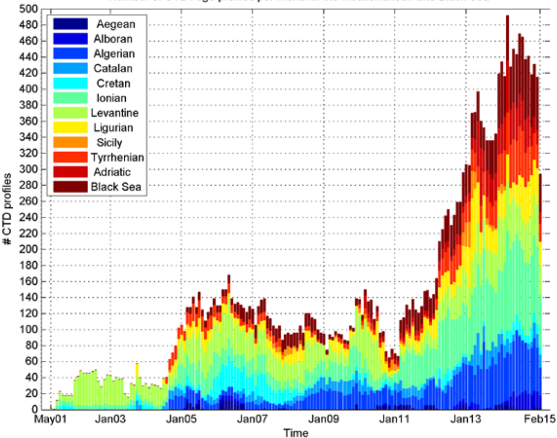
Number of CTD Argo profiles per month in the Mediterranean and Black Sea
